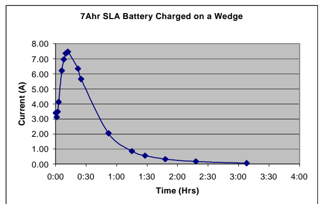
Battery Charging Curve
